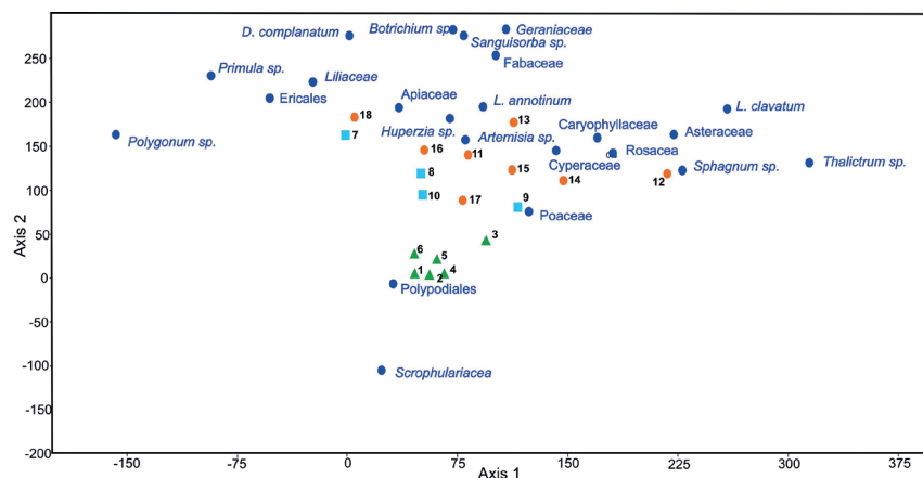
Figure 7 DCA biplot for main pollen taxa (blue circle), Onkotan Island. Symbols indicate vegetation types: triangle – shrub thicket; square – dwarf shrub–tundra-like; red circle – meadow
