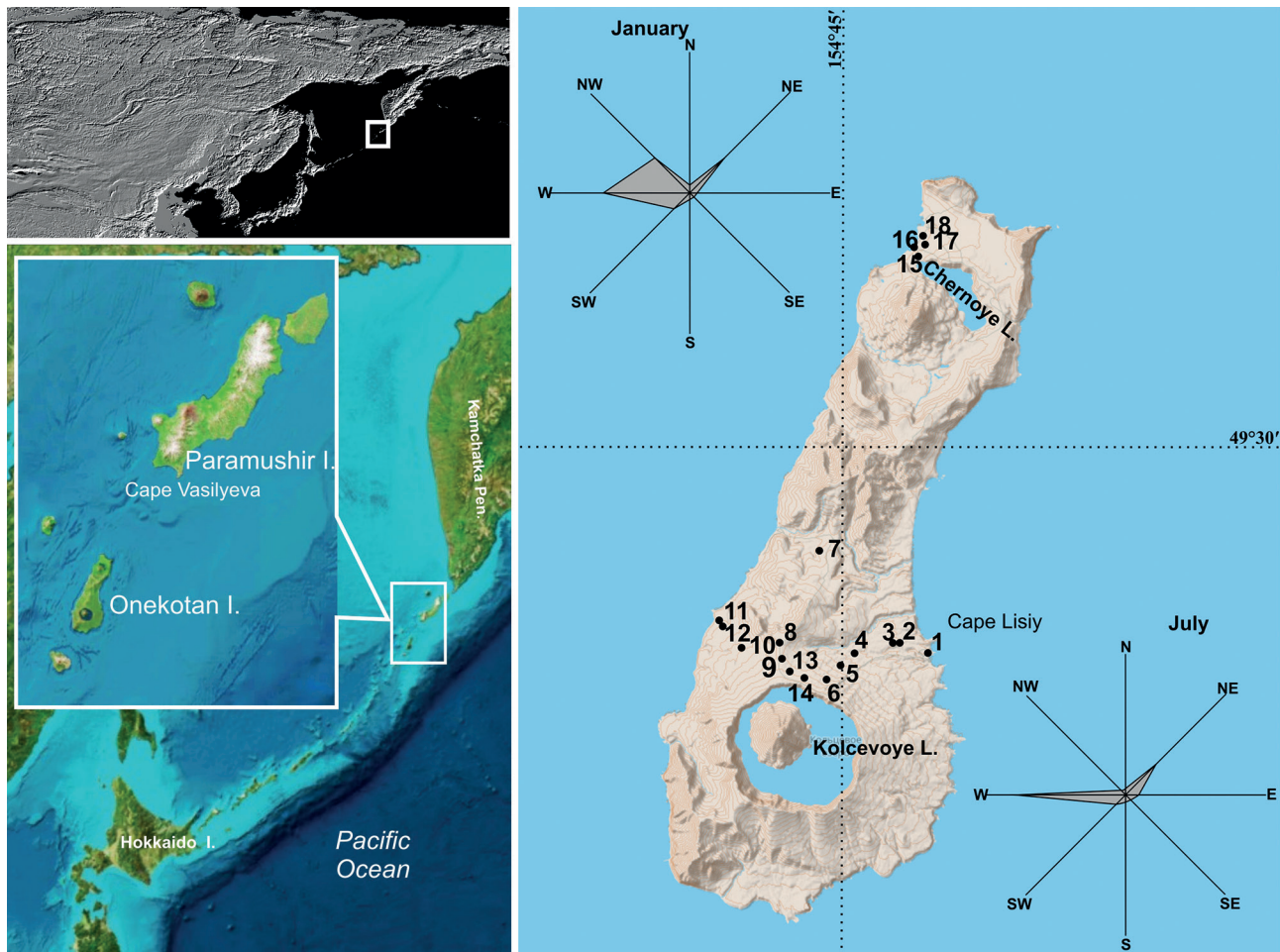
Figure 1 Location map of sampling sites for modern sediment samples analyzed by pollen analysis on Onkotan Island. Base map from www.ru-topographic-map.com . Wind rose constructed from data of the nearest weather station (Vasilyeva Cape)
