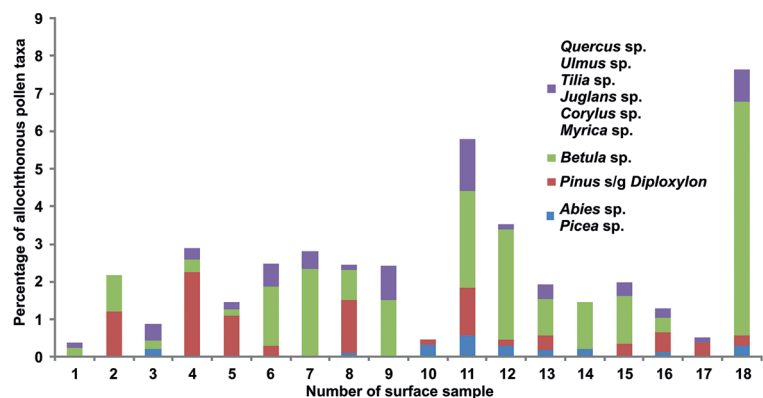
Figure 4 Percentage of allochthonous pollen taxa in subfossil deposits on Onkotan Island
