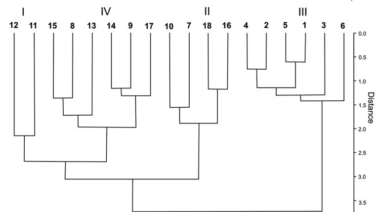
Figure 5 Hierarchical cluster analysis of pollen and spore assemblages from 18 surface samples on Onkotan Island. Bootstrap support values (%) are based on 2 000 replicates. The cophenetic correlation coefficient was 0.57; agreement between Ward clustering and independent k-means classification was moderate (ARI = 0.664)
