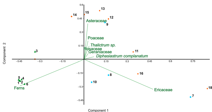
Figure 6 PCA biplot for main pollen taxa, Onkotan Island. Symbols indicate vegetation types: triangle – shrub thicket; square – dwarf shrub–tundra-like; circle – meadow
