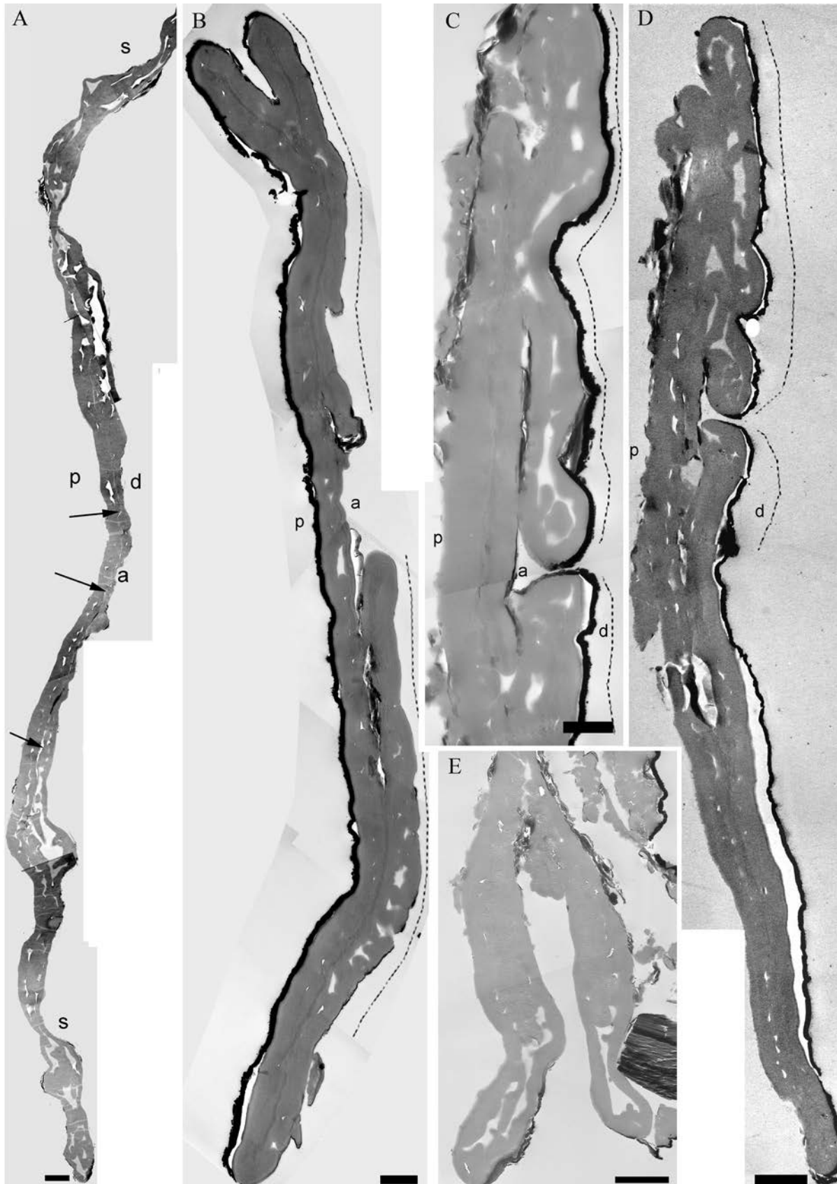
Figure 1 Ultrathin sections of pollen of Vesicaspora sp. and Antesia zeilleri (Nathorst) Harris 1937 (illustrations are reproduced from Zavialova 1998 and Zavialova & Van Konijnenburg-van Cittert 2011). A. Pollen of Vesicaspora sp., composite longitudinal section through the body and sacci, proximal face to the left, arrows point to the obliterated gametophyte hollow. B–E. Pollen of A. zeilleri . B. Composite section shows thinned ectexine in the apertural region and extensions of the exine bordering the aperture, proximal face to the left. C. Enlargement of D. D. Composite section of a pollen grain, proximal exine shows regular alveolae, distal-equatorial extensions surround the aperture. E. Section of a pollen grain compressed in lateral position, distal face to the bottom of the figure. Scale bars (A, D, E) 1 \mu\text{m} , (B, C) 0.67 \mu\text{m} ; (a) aperture, (d) distal face, (p) proximal face, (s) saccus, intermittent line indicates the position of extensions surrounding the aperture
